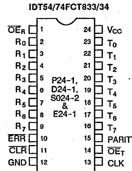
DIP/SOIC/CERPACK TOP VIEW
