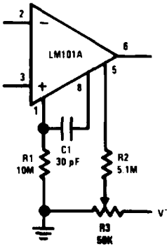
Standard Compensation and Offset Balancing Circuit
