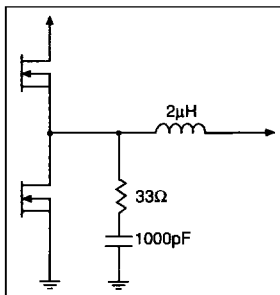
Figure 18: Filter components
