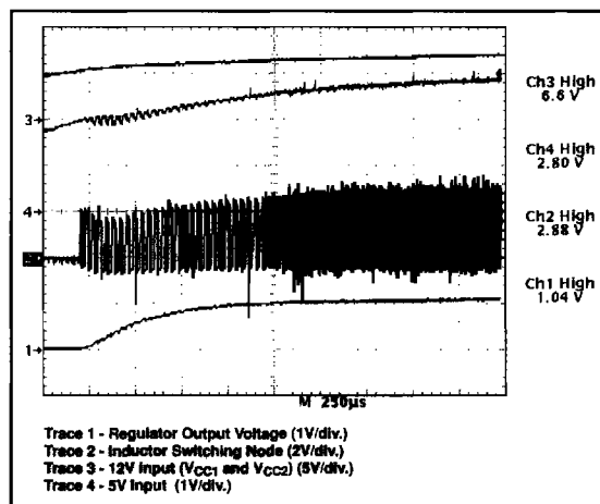
Figure 2: CS-5150 demonstration board startup in response to increasing 12V and 5V input voltages. Extended off time is followed by normal off time operation when output voltage achieves regulation to the error amplifier output.
