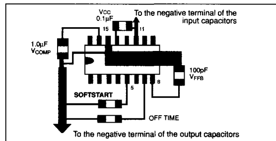
Figure 20: Layout Guidelines
