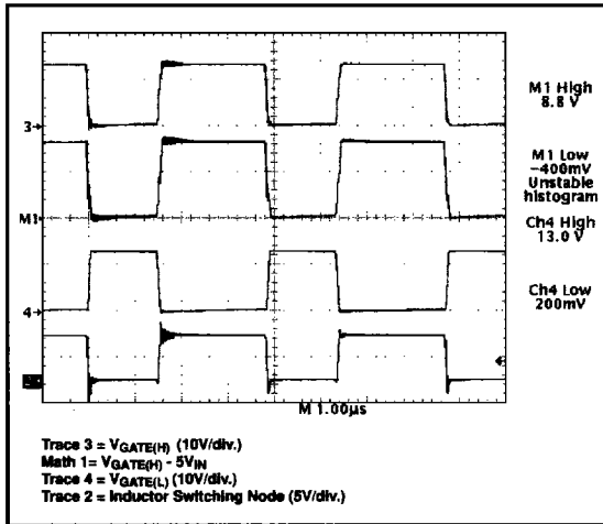
Figure 17: CS-5150 gate drive waveforms depicting tail to rail swing.
