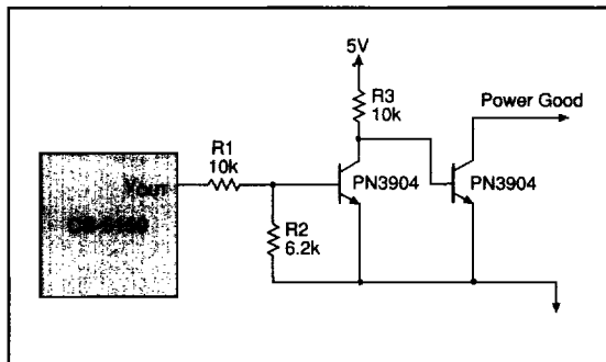
Figure 15: Implementing Power Good with the CS-5150.
