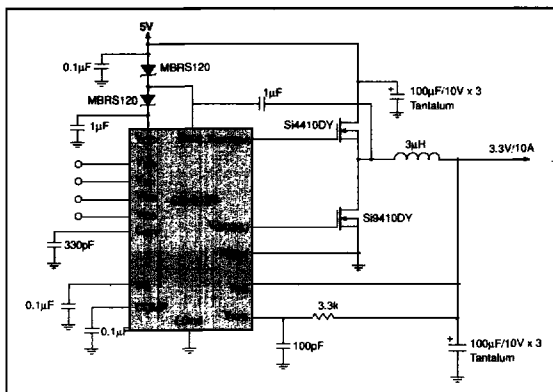
Figure 21: 5V to 3.3V/10A converter.
