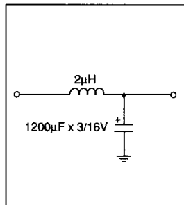
Figure 19: Input Filter
