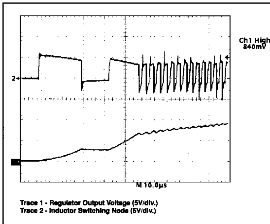
Figure 4: CS-5150 demonstration board enable startup waveforms.
