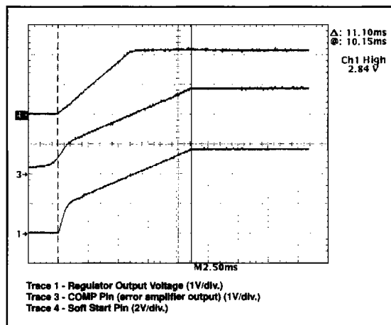
Figure 3: CS-5150 demonstration board startup waveforms.
