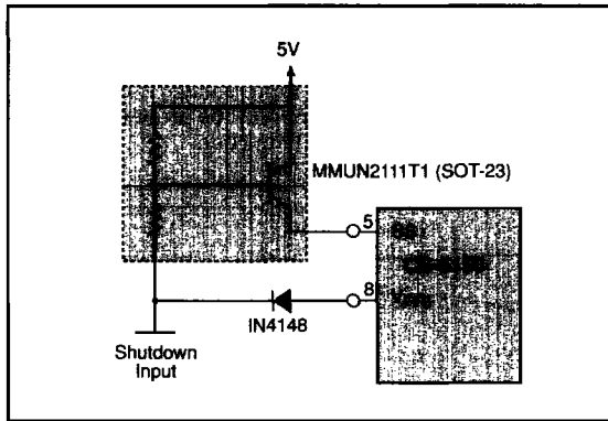
Figure 14: Implementing shutdown with the CS-5150.
