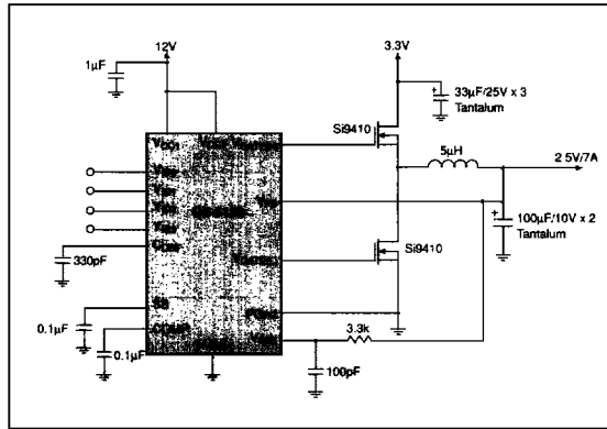
Figure 24: 3.3V to 2.5V/7A converter with 12V bias.
