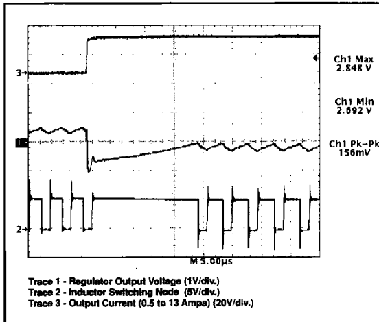
Figure 8: CS-5150 demonstration board response to 13A load turn on (output set for 2.8V). Upon completing a normal off time, the V^2 control loop immediately connects the inductor to the input voltage, providing 100% duty cycle. Regulation is achieved in less than 20µs.
