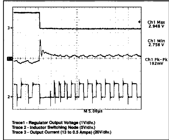
Figure 9: CS-5150 demonstration board response to 13A load turn off (output set for 2.8V). V^2 control topology immediately connects inductor to ground, providing 0% duty cycle. Regulation is achieved in less than 10µs.
