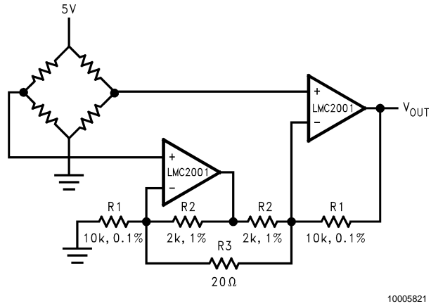
FIGURE 4. Single Supply Strain- Gauge Amplifier
