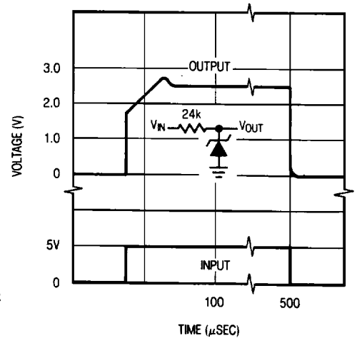
Response Time
