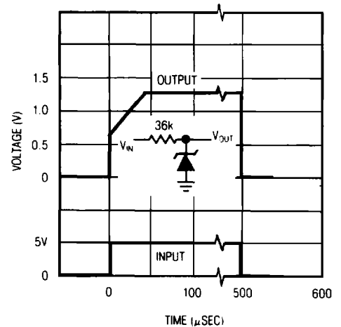
Response Time
