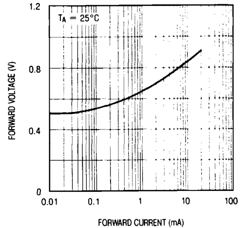
Forward Characteristics
