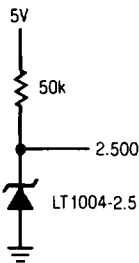
2.5V Reference
