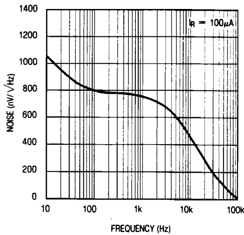
Noise Voltage
