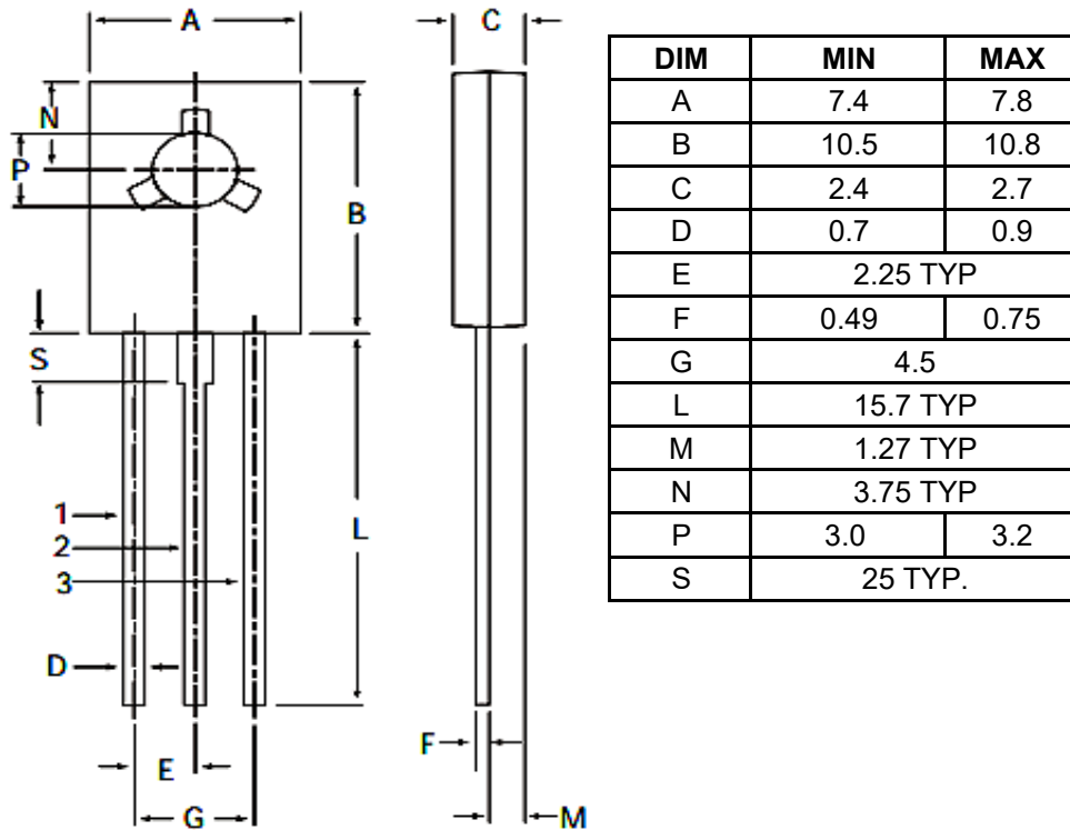
TO-126 Leaded Plastic Package
