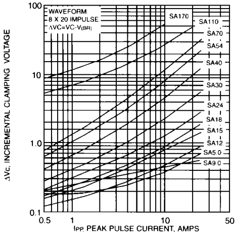
FIG. 6 - INCREMENTAL CLAMPING VOLTAGE CURVE UNIDIRECTIONAL
