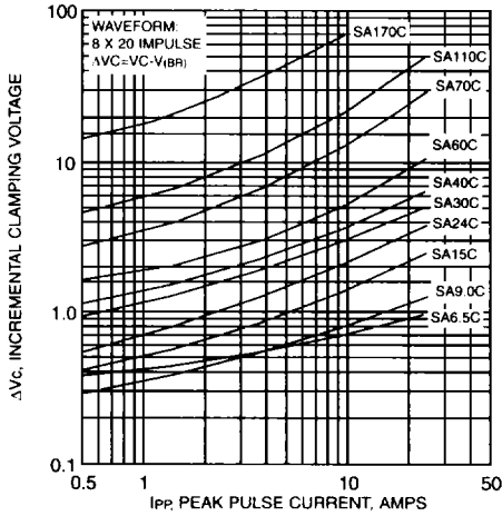
FIG. 8 - INCREMENTAL CLAMPING VOLTAGE CURVE BIDIRECTIONAL
