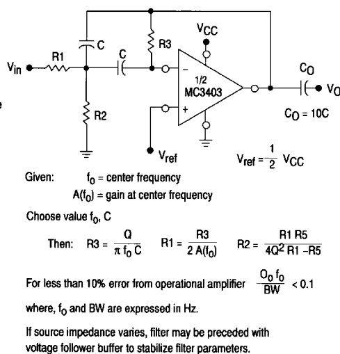
Figure 13. Multiple Feedback Bandpass Filter
