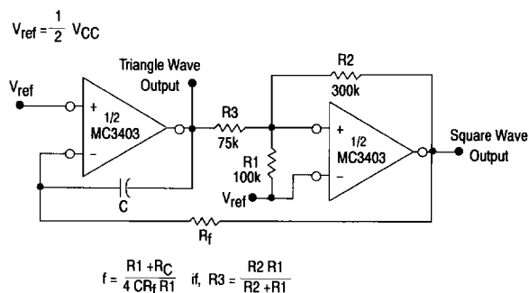
Figure 12. Function Generator
