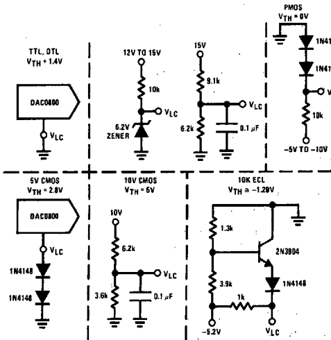
FIGURE 11. Interfacing with Various Logic Families
