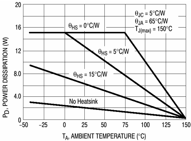
FIGURE 1 - WORST CASE POWER DISSIPATION VERSUS AMBIENT TEMPERATURE
