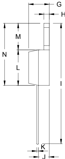
2.Side View
