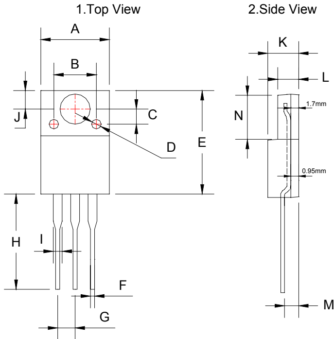
TO-220F Mechanical drawing
