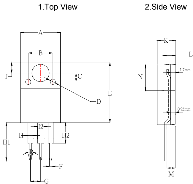
TO-220FS Mechanical drawing
