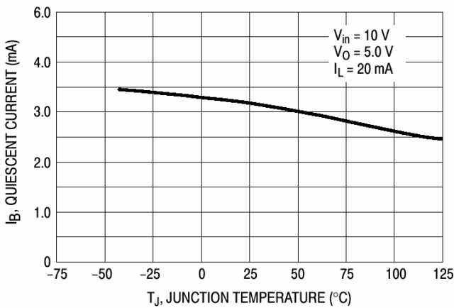
FIGURE 3 - QUIESCENT CURRENT AS A FUNCTION OF TEMPERATURE
