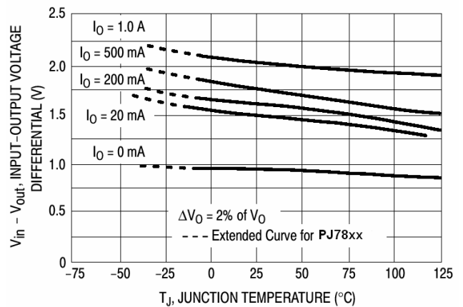
FIGURE 4 - INPUT OUTPUT DIFFERENTIAL AS A FUNCTION OF JUNCTION TEMPERATURE
