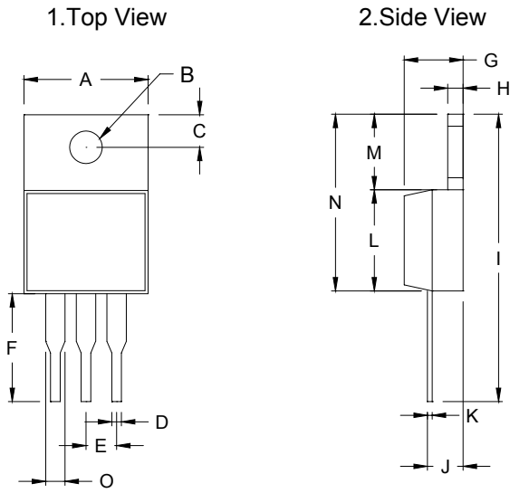
TO-220S Mechanical drawing
