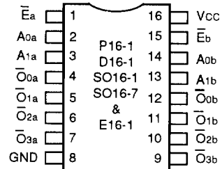
DIP/SOIC/QSOP/CERPACK TOP VIEW
