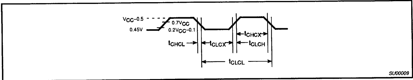
Figure 23. Clock Signal Waveform for I_{CC} Tests in Active and Idle Modes t_{CLCH} = t_{CHCL} = 5\text{ns}
