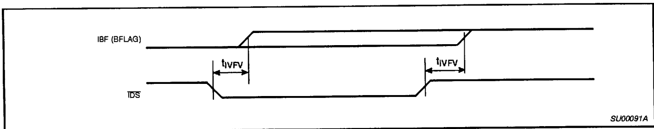
Figure 16. IBF Flag Output
