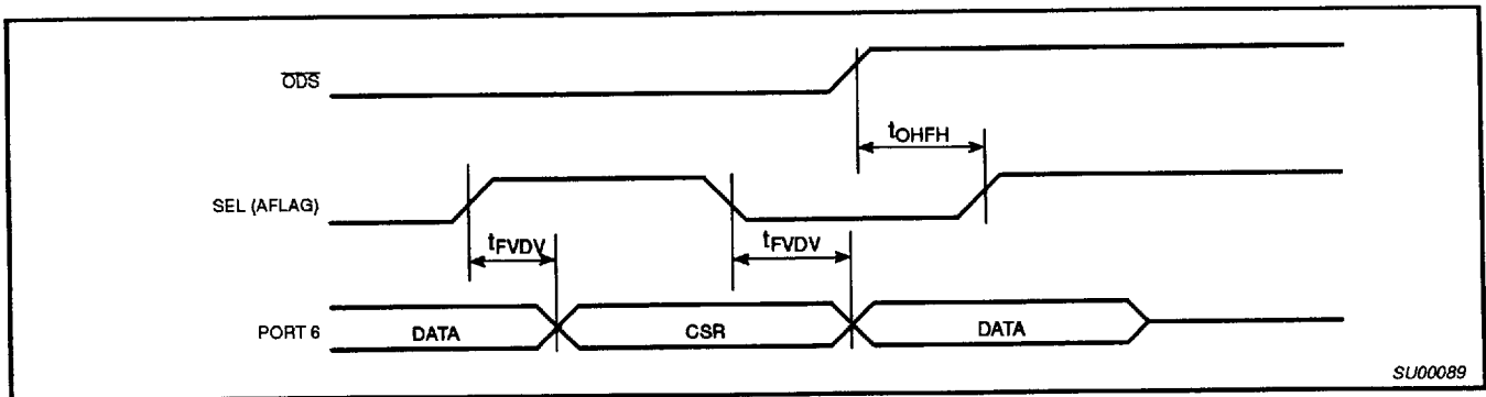
Figure 14. Port 6 Select Mode
