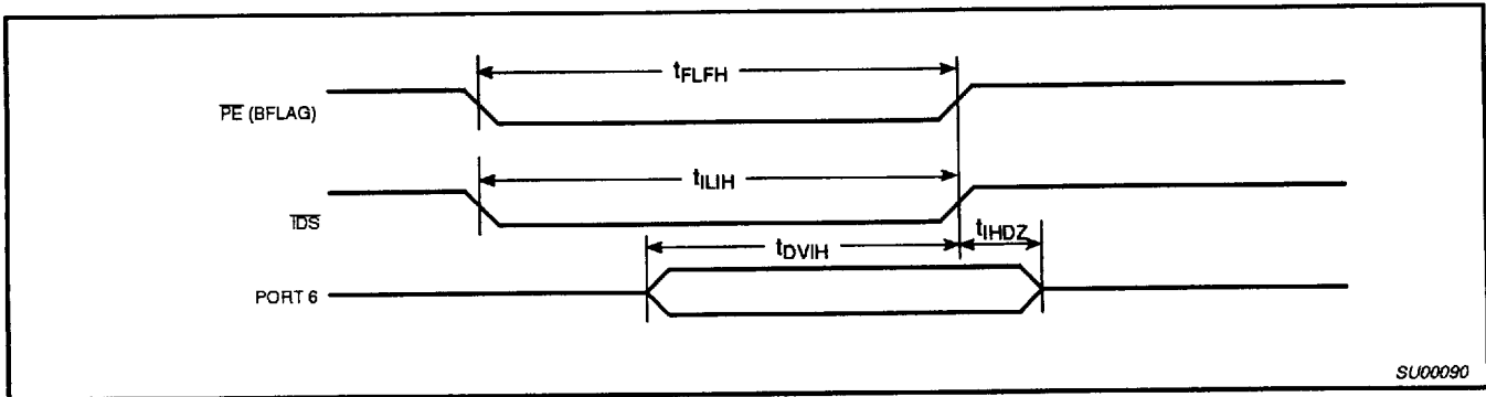
Figure 15. Port 6 Input
