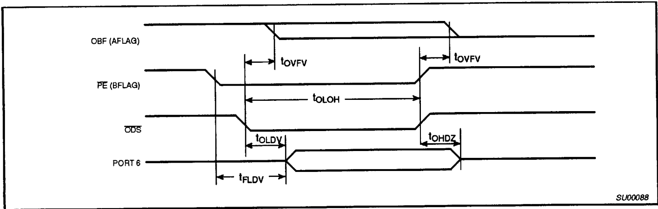
Figure 13. Port 6 Output
