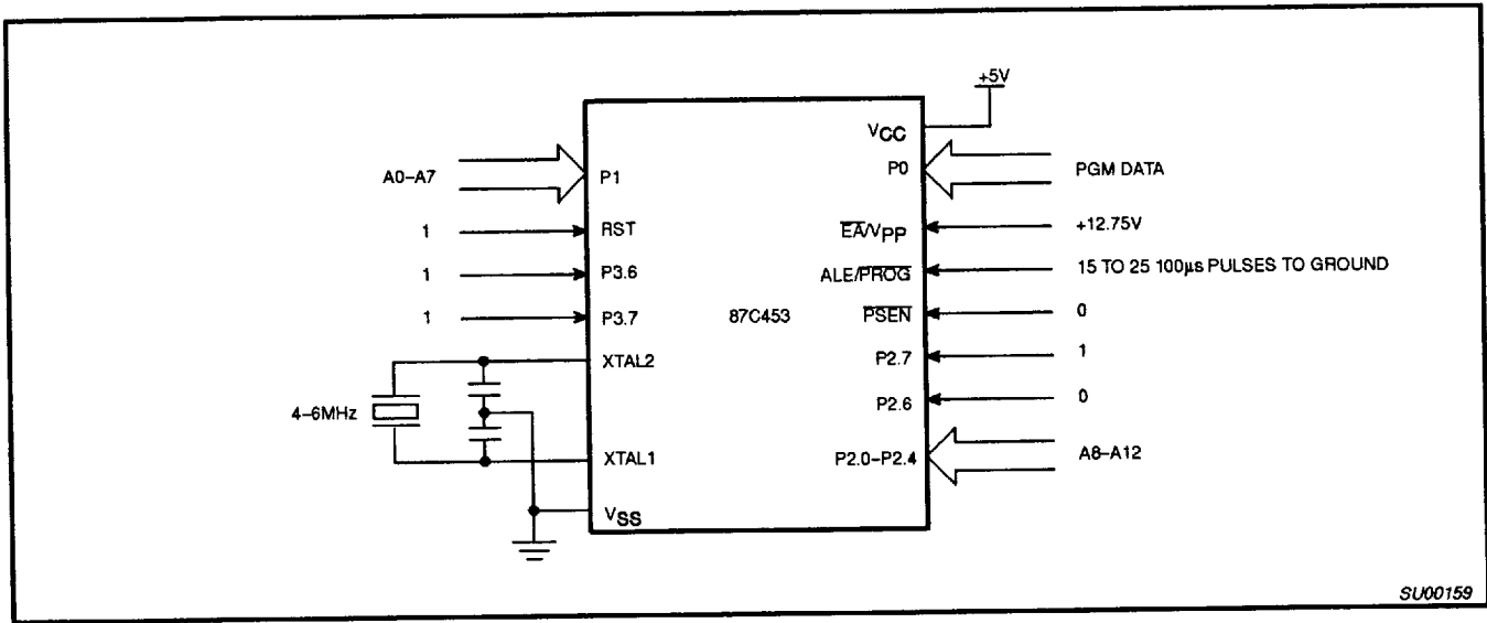
Figure 25. Programming Configuration
