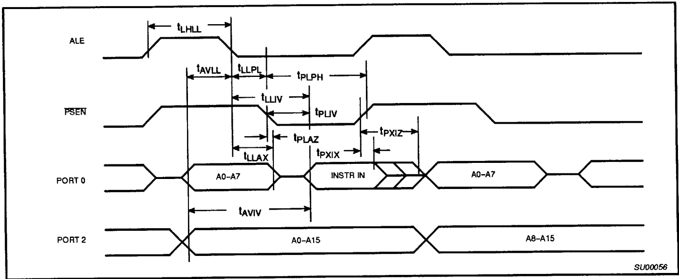
Figure 9. External Program Memory Read Cycle
