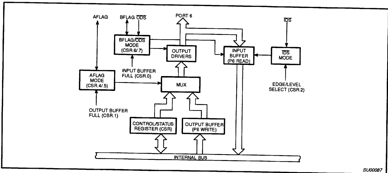
Figure 8. Port 6 Block Diagram
