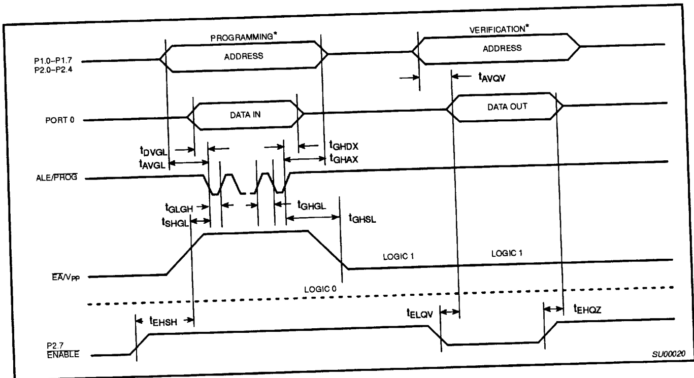
Figure 28. EPROM Programming and Verification
