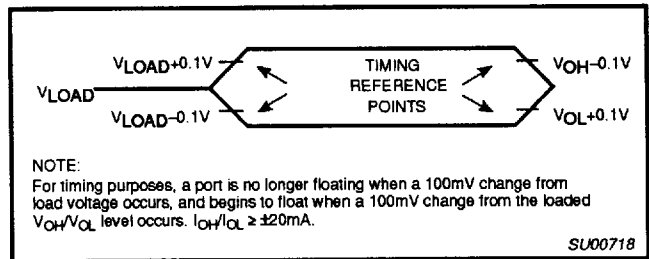
Figure 19. Float Waveform
