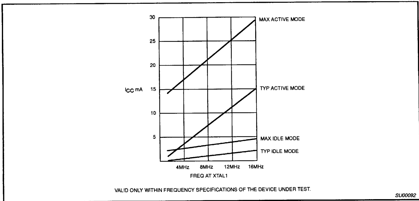
Figure 20. I_{CC} vs. FREQ
