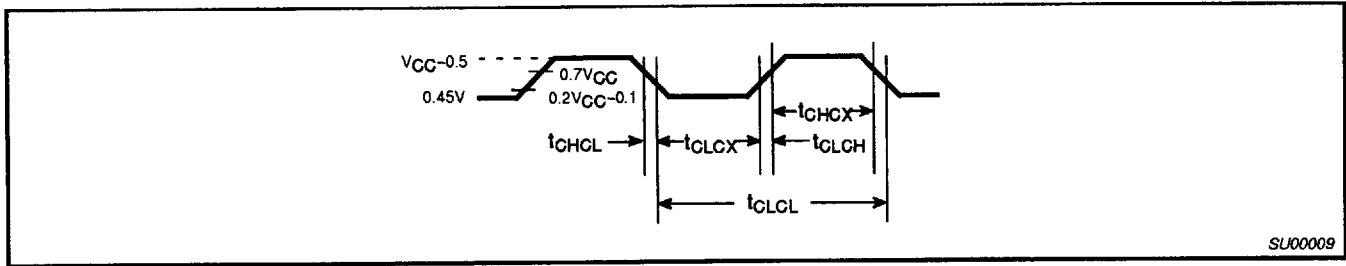
Figure 17. External Clock Drive
