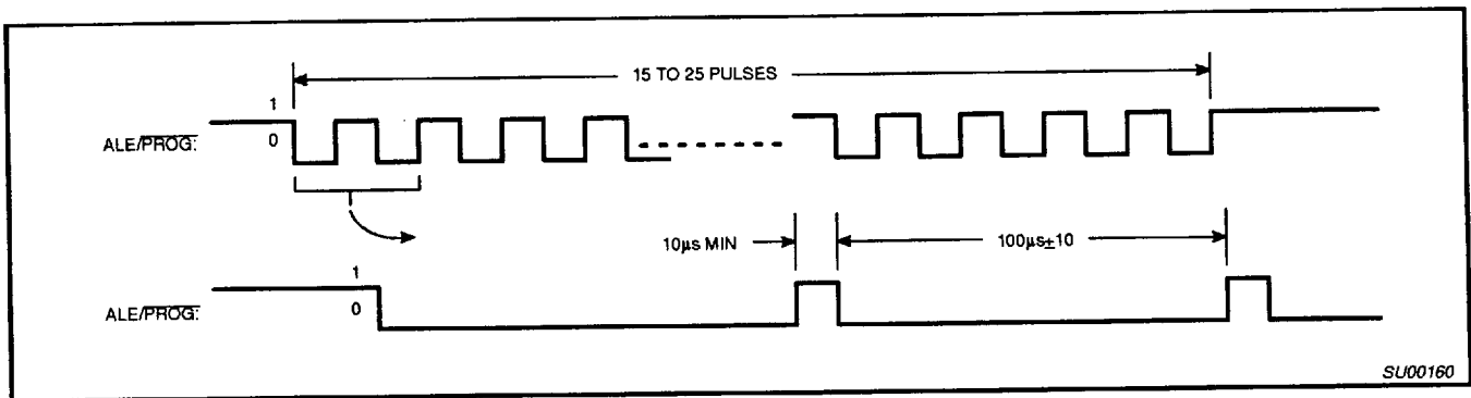
Figure 26. PROG Waveform
