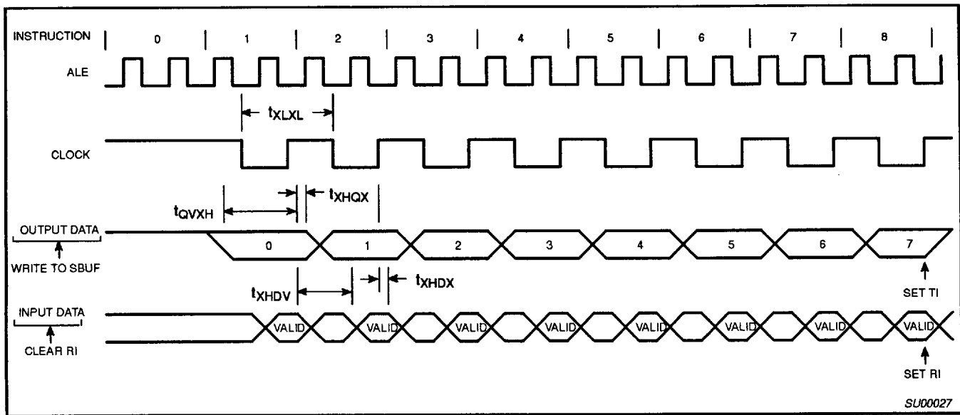
Figure 12. Shift Register Mode Timing
