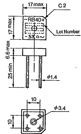
Outline Drawing ⑤③
