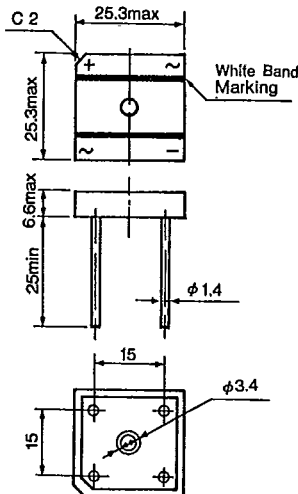
Outline Drawing ⑤④
