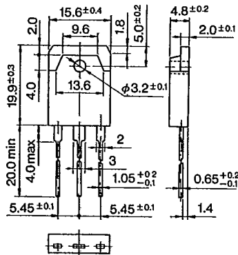
Outline Drawing ⑤①
