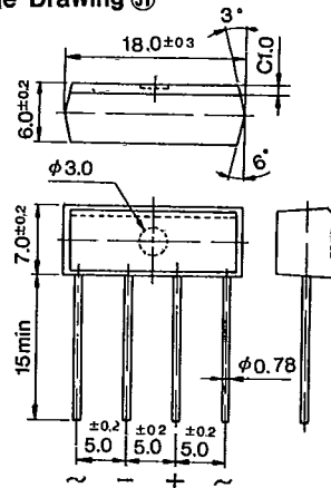
Outline Drawing ⑤②
