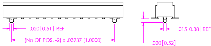
FIG 5 -A: MOLDED ALIGNMENT PIN
