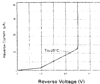
Reverse Characteristics
