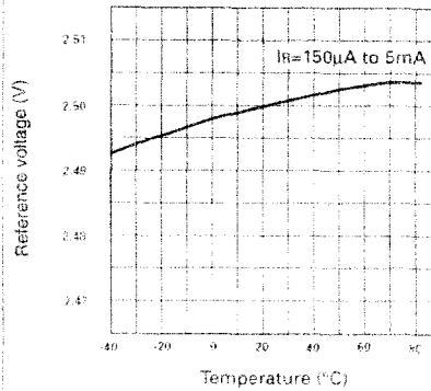
Temperature Drift
