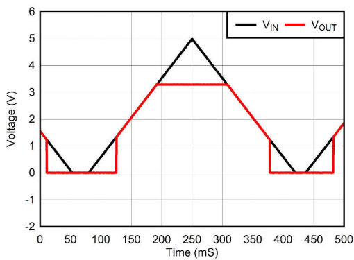
Figure 5-37. TPS73701, V_{OUT} = 3.3\text{-V} Power-Up and Power-Down
