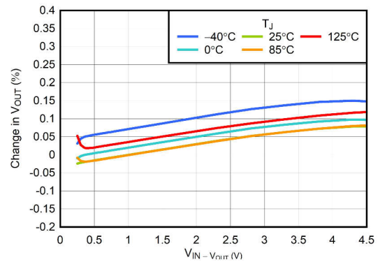
New silicon, M3 suffix Figure 5-4. Line Regulation
