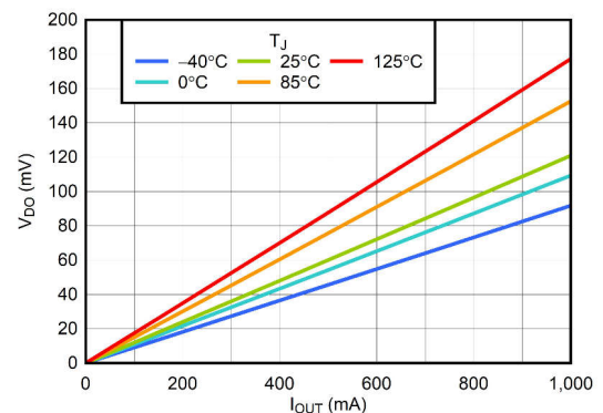
New silicon, M3 suffix Figure 5-6. Dropout Voltage vs Output Current
