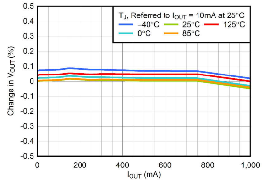
New silicon, M3 suffix Figure 5-2. Load Regulation
