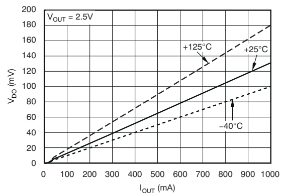
Legacy silicon Figure 5-5. Dropout Voltage vs Output Current
