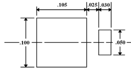
MOUNTING PAD
