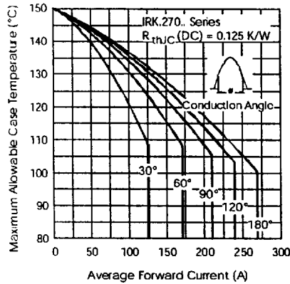
Fig. 12-Current Ratings Characteristics
