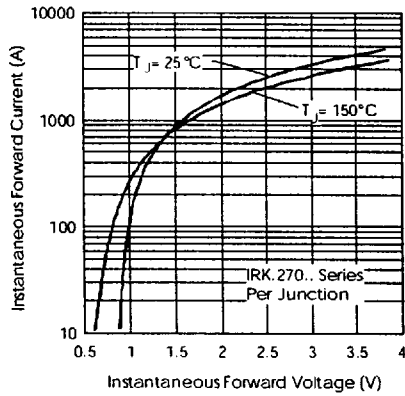
Fig.21-Forward Voltage Drop Characteristics
