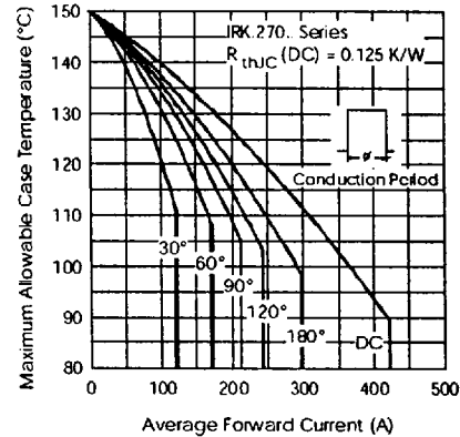
Fig. 13-Current Ratings Characteristics
