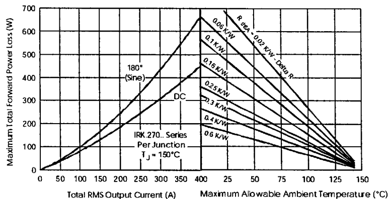
Fig. 16 - Forward Power Loss Characteristics
