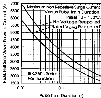
Fig. 9 - Maximum Non-Repetitive Surge Current
