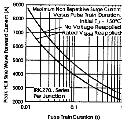
Fig. 20 - Maximum Non-Repetitive Surge Current
