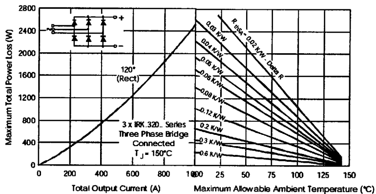
Fig. 29 - Forward Power Loss Characteristics
