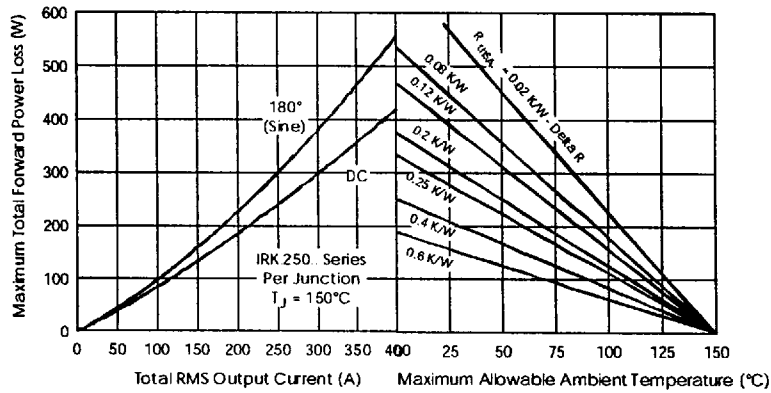
Fig.5-ForwardPowerLossCharacteristics
