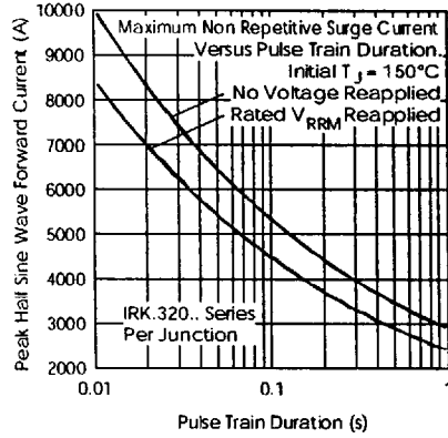
Fig.31-Maximum Non-Repetitive Surge Current
