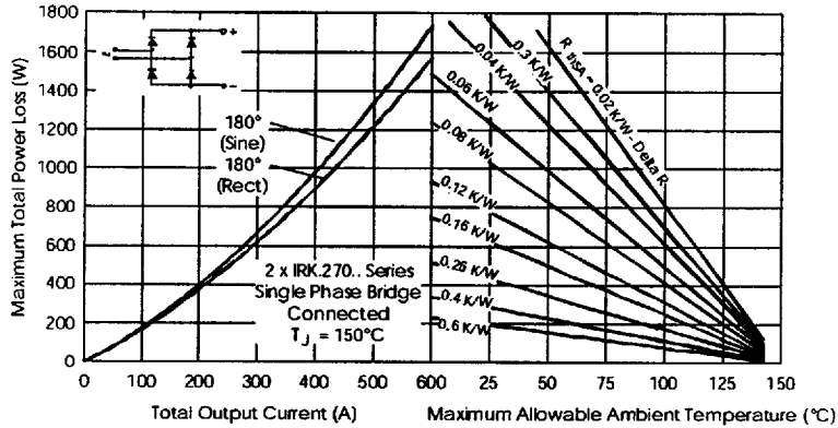
Fig. 17 - Forward Power Loss Characteristics
