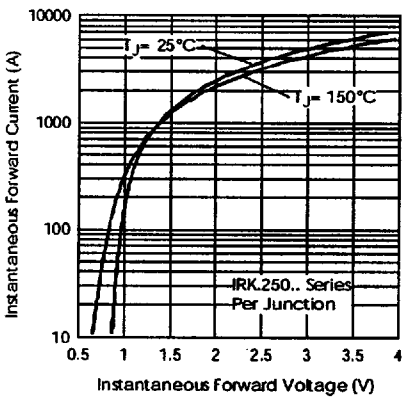
Fig. 10 - Forward Voltage Drop Characteristics
