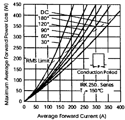
Fig.4-ForwardPowerLossCharacteristics
