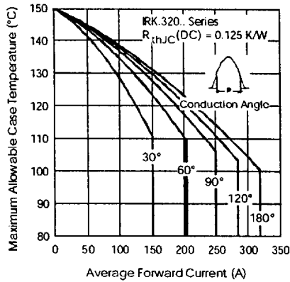
Fig.23-Current Ratings Characteristics
