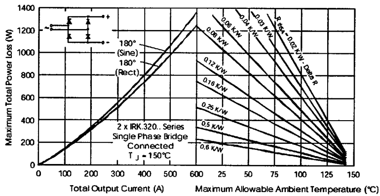
Fig. 28-ForwardPowerLossCharacteristics
