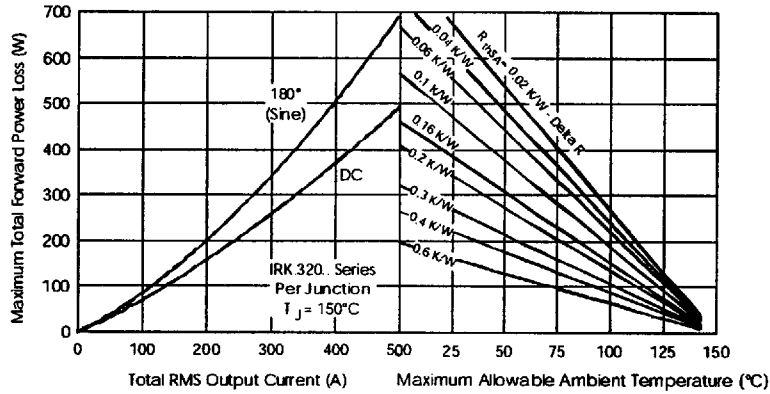
Fig. 27-ForwardPowerLossCharacteristics
