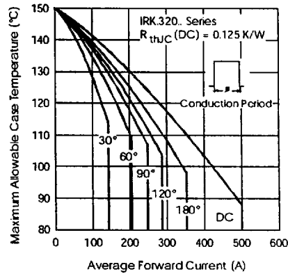
Fig.24-Current Ratings Characteristics
