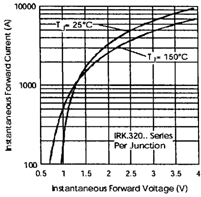
Fig.32-Forward Voltage Drop Characteristics
