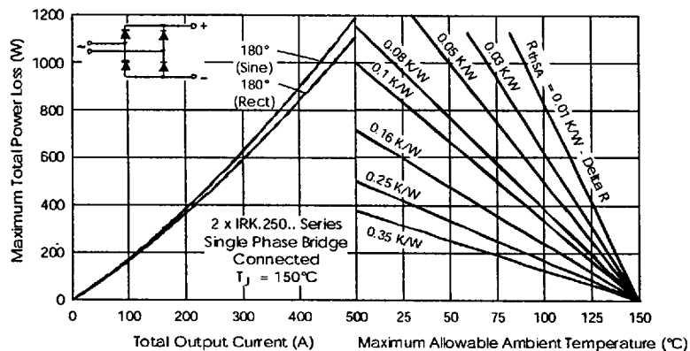
Fig. 6 - Forward Power Loss Characteristics
