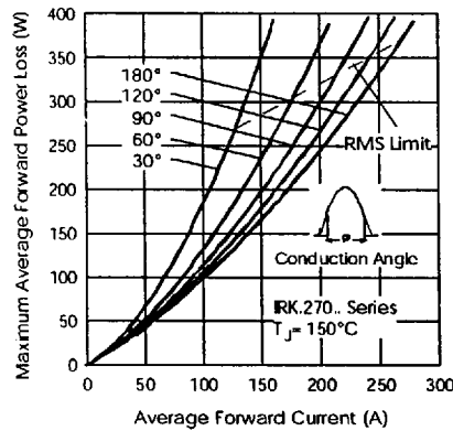
Fig. 14-Forward Power Loss Characteristics
