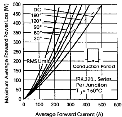
Fig. 26 - Forward Power Loss Characteristics
