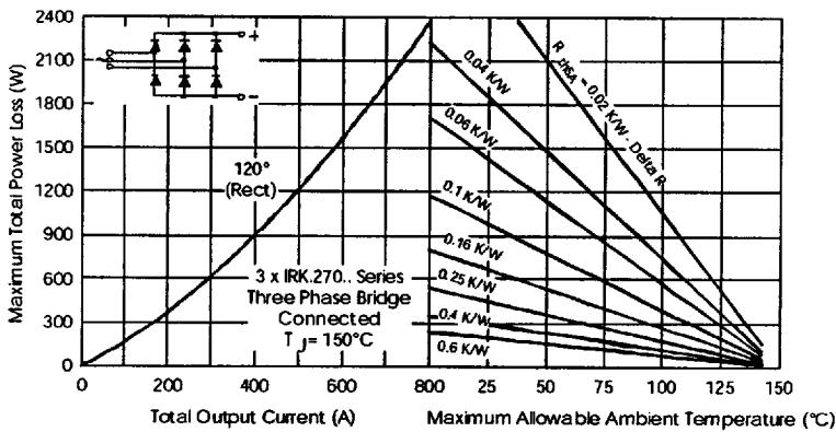
Fig. 18 - Forward Power Loss Characteristics
