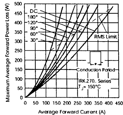
Fig. 15-Forward Power Loss Characteristics
