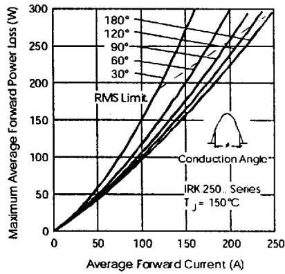
Fig.3-ForwardPowerLossCharacteristics
