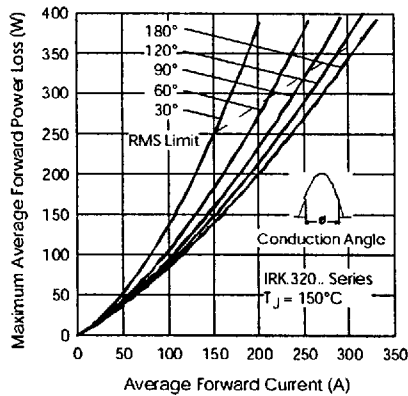
Fig. 25 - Forward Power Loss Characteristics
