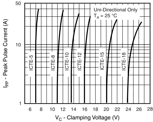
Figure 7. Typical Characteristics Clamping Voltage
