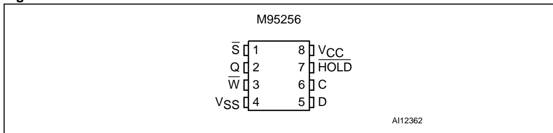
Figure 2. SO and TSSOP connections
