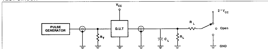
Test Circuit
