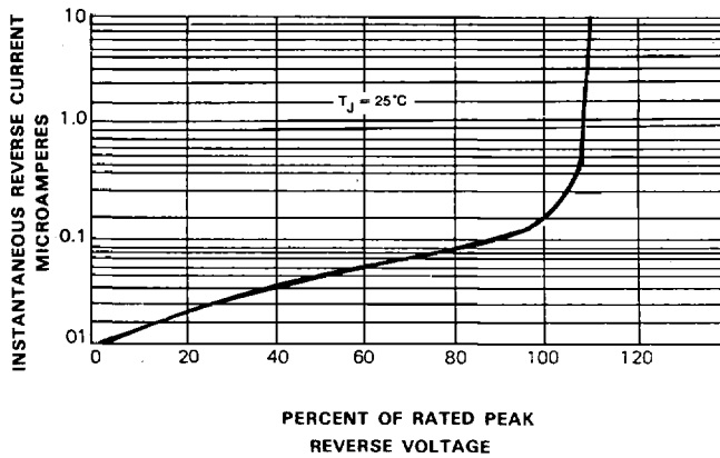
FIG. 4. TYPICAL REVERSE CHARACTERISTIC
