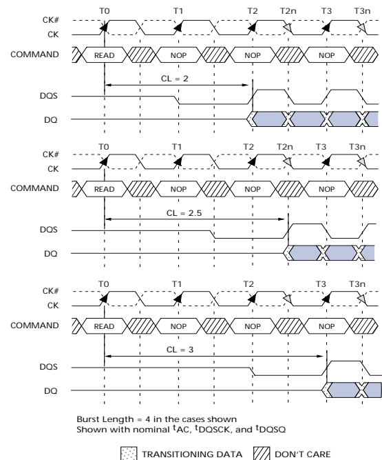
Figure 8: CAS Latency
