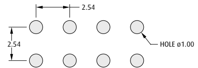
Recommended PC Board Pattern
