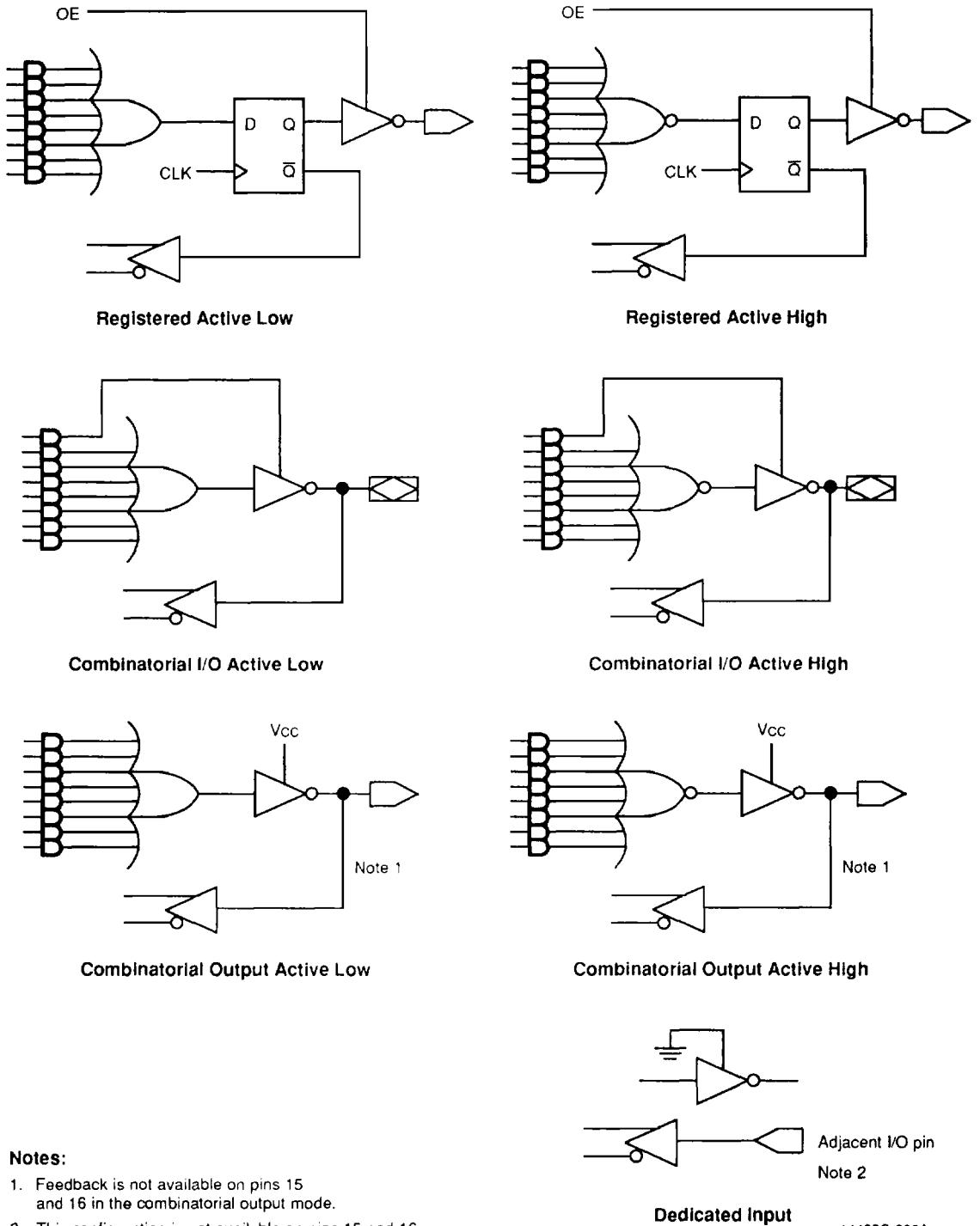
Figure 2. Macrocell Configurations
