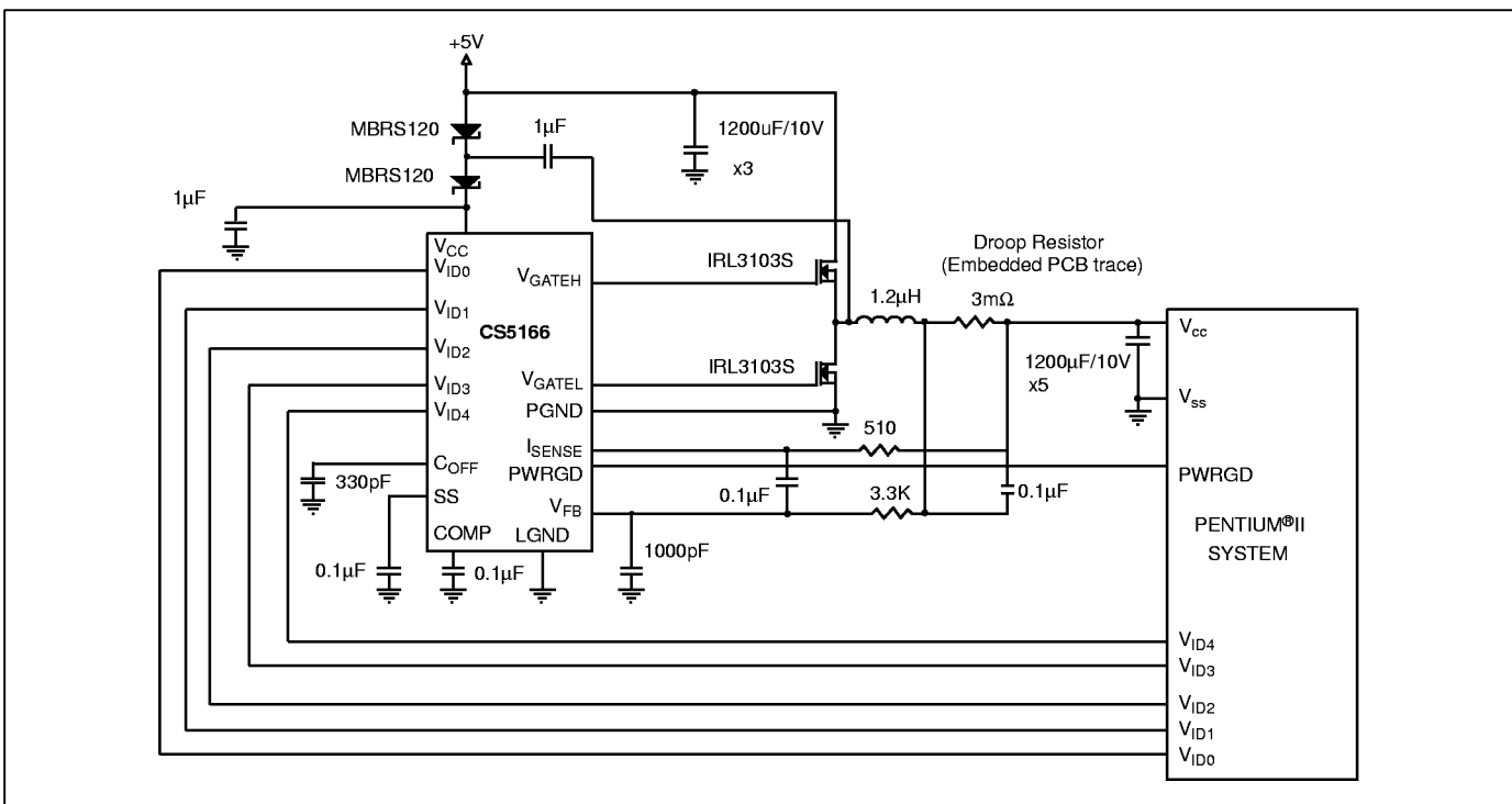
Figure 37: +5V to +2.8V @ 14.2A for 300 MHz Pentium® II.
