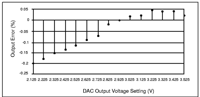
Figure 35: Percent Output Error vs. DAC Output Voltage Setting V_{CC} = 12V , T_A = 25^{\circ}C , V_{ID4} = 1 .
