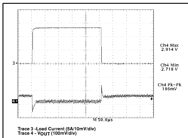
Figure 8: Output Voltage Transient Response to a 14A load pulse, V_{OUT} = 2.825V (DAC = 10111).
