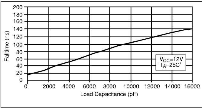
Figure 31: GATE(H) & GATE(L) Falltime vs. Load Capacitance.
