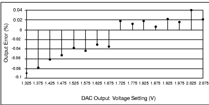
Figure 32: Percent Output Error vs DAC Voltage Setting, V_{CC} = 12V , T_A = 25^{\circ}C , V_{ID4} = 0 .
