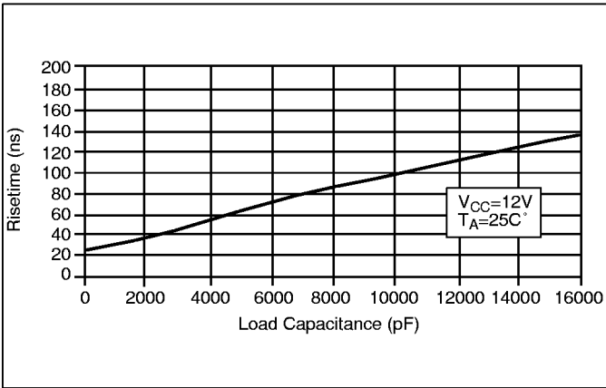
Figure 30: GATE(L) Risettime vs. Load Capacitance.
