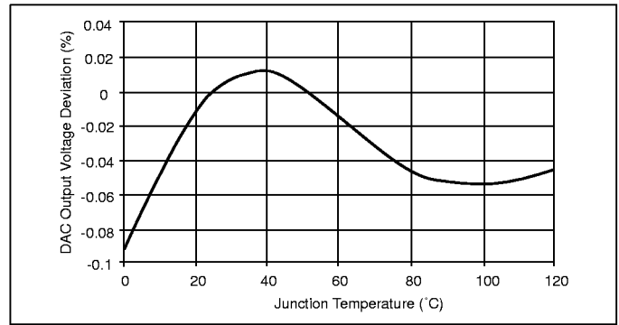
Figure 34: DAC Output Voltage vs Temperature, DAC Code = 10111, V_{CC} = 12V .
