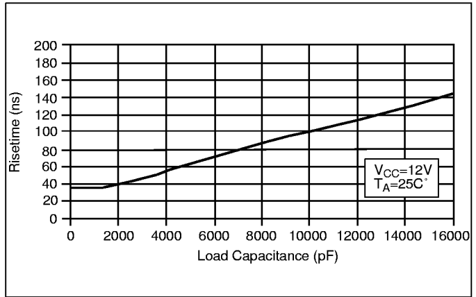
Figure 33: GATE(H) Risettime vs. Load Capacitance.
