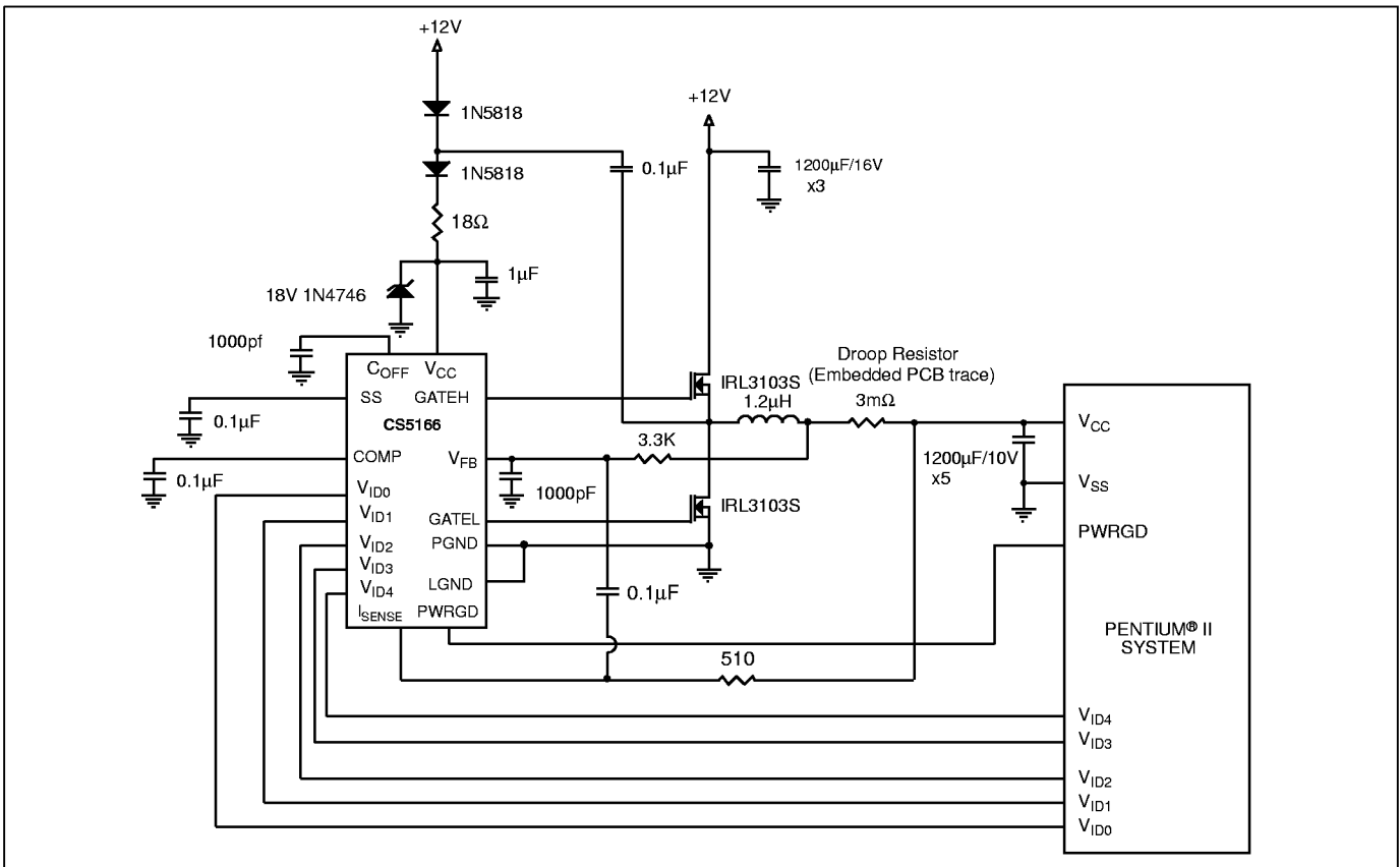
Figure 36: +12V to +2.8V @ 14.2A for 300 MHz Pentium® II.
