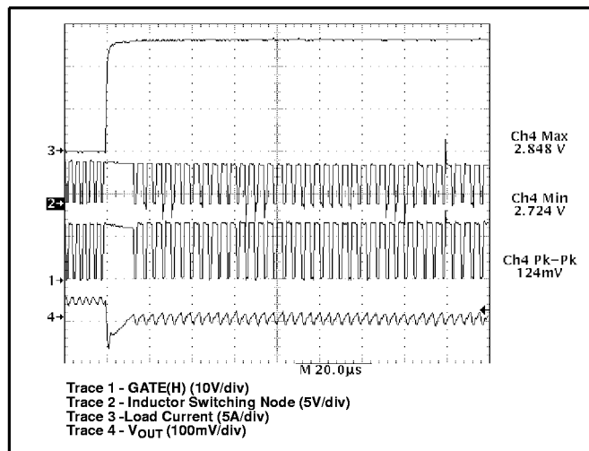
Figure 9: Output Voltage Transient Response to a 14A load step, V_{OUT} = 2.825V (DAC = 10111).
