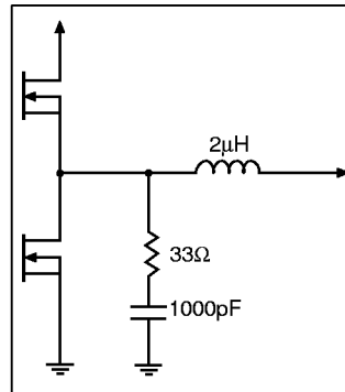
Figure 27: Filter components.
