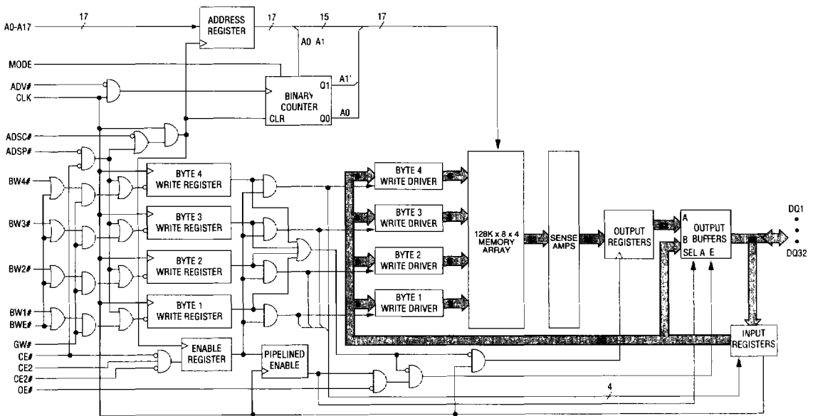
FUNCTIONAL BLOCK DIAGRAM 128K x 32
