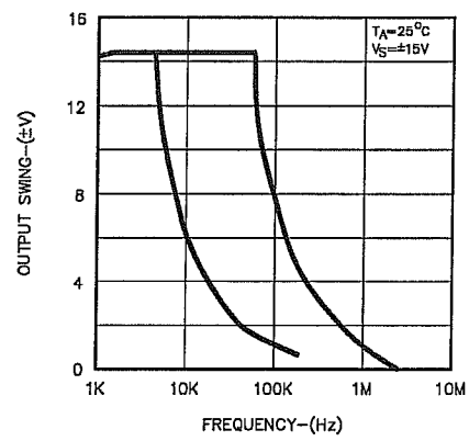
FIGURE 8. LARGE SIGNAL FREQUENCY RESPONSE
