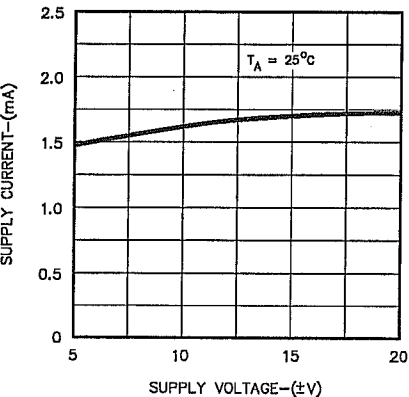
FIGURE 4. SUPPLY CURRENT VS. SUPPLY VOLTAGE
