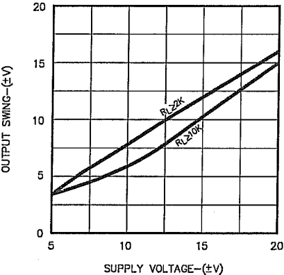
FIGURE 2. OUTPUT SWING VS. SUPPLY VOLTAGE
