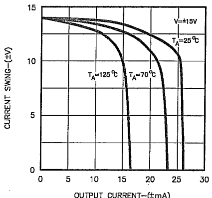
FIGURE 6. CURRENT LIMITING
