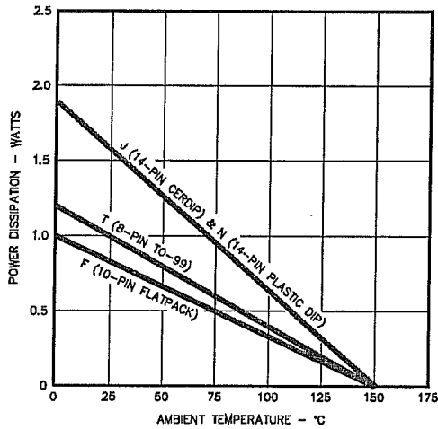
MAXIMUM POWER DISSIPATION vs AMBIENT TEMPERATURE
