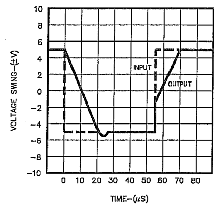
FIGURE 9. VOLTAGE FOLLOWER PULSE RESPONSE
