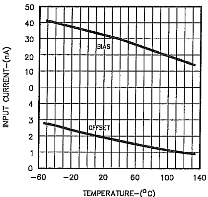
FIGURE 5. INPUT CURRENT VS. TEMPERATURE
