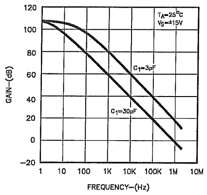
FIGURE 7. OPEN LOOP FREQUENCY RESPONSE
