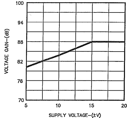
FIGURE 3. MINIMUM VOLTAGE GAIN
