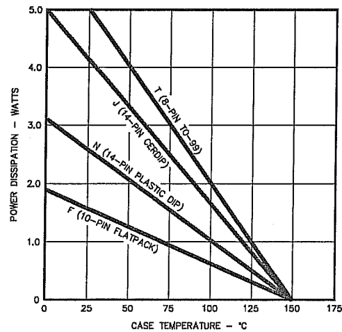
MAXIMUM POWER DISSIPATION vs CASE TEMPERATURE
