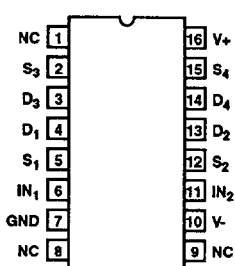
DG303ACY (SOIC) TOP VIEW
