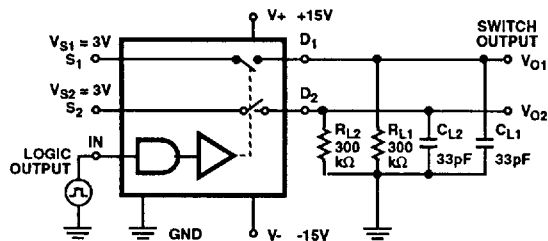
FIGURE 2. BREAK-BEFORE MAKE TEST CIRCUIT (DG301A, DG303A)
