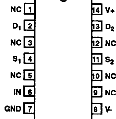
DG301A (CDIP, PDIP) TOP VIEW
