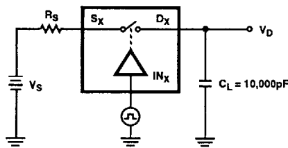
FIGURE 1. CHARGE INJECTION TEST CIRCUIT
