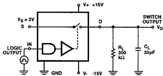
FIGURE 3. t_{ON} and t_{OFF} TEST CIRCUIT
