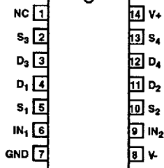
DG302A (CDIP, PDIP) TOP VIEW
