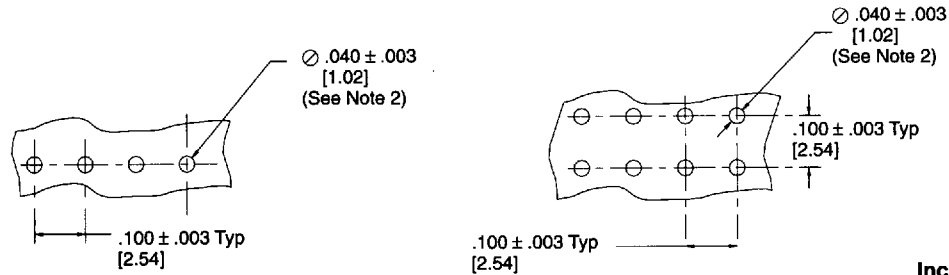
Recommended Mounting Hole Pattern
