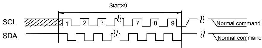
Fig.48-(c) START×9+ command input
