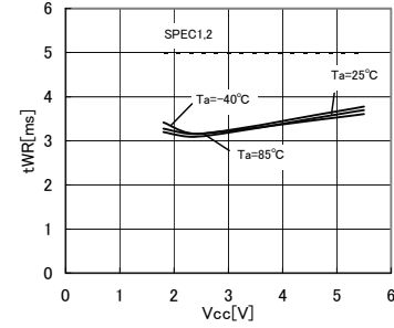
Fig.28 Internal write cycle time tWR
