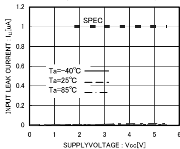
Fig.7 Input leak current I_{II} (A0,A,A2,SCL,WP)
