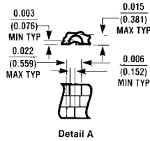
Ceramic Leadless Chip Carrier Package (E) Order Number 54LS09LMQB Package Number E20A
