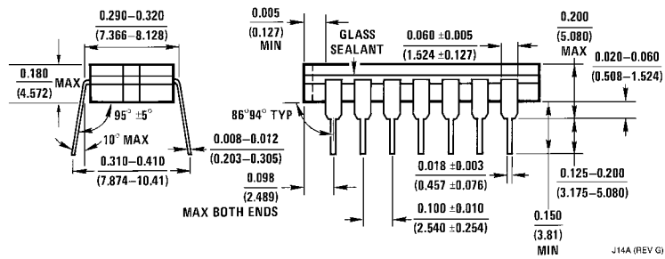
14-Lead Ceramic Dual-In-Line Package (J) Order Number 54LS09DMQB or DM54LS09J Package Number J14A
