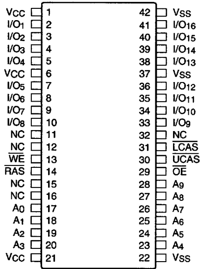
42-Pin Plastic SOJ PIN CONFIGURATION Top View
