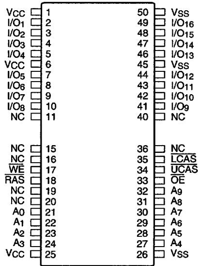
44/50-Pin Plastic TSOP-II PIN CONFIGURATION Top View
