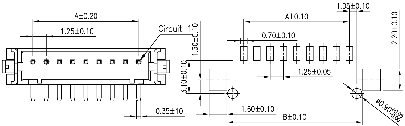
PCB LAYOUT
