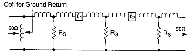
Figure 7. High Power Equivalent Circuit
