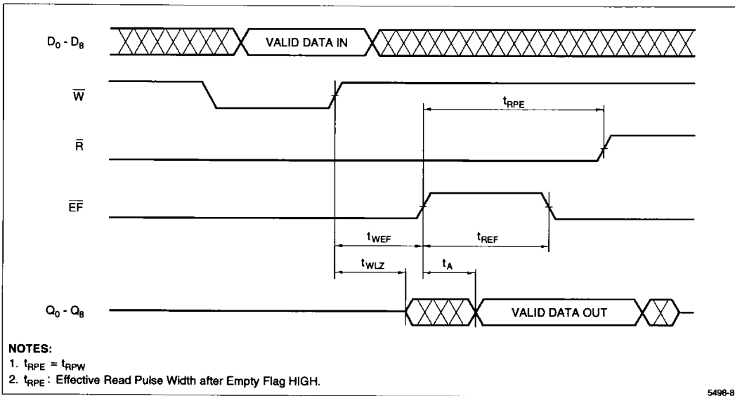
Figure 9. Read Data Flow-Through
