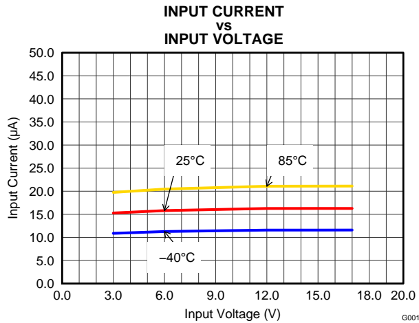
Figure 17. Quiescent Current
