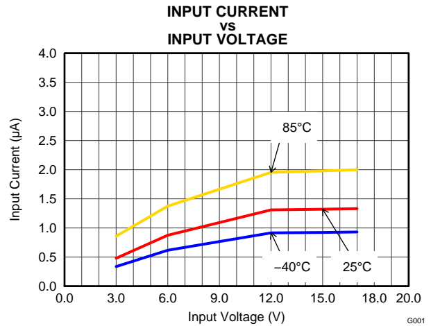
Figure 18. Shutdown Current
