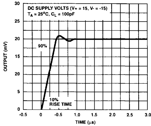
FIGURE 5. TRANSIENT RESPONSE FOR CA741C AND CA741
