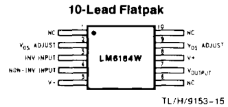
Top View NS Package Number W10A
