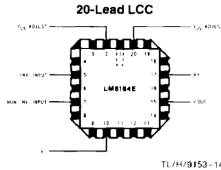
Top View NS Package Number E20A
