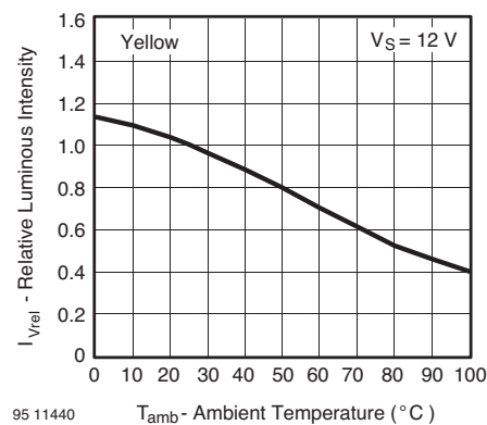
Figure 17. Rel. Luminous Intensity vs. Ambient Temperature
