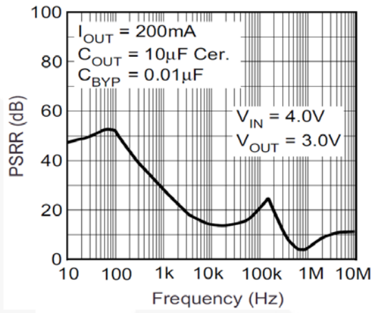
Figure 10. Power Supply Rejection Ratio
