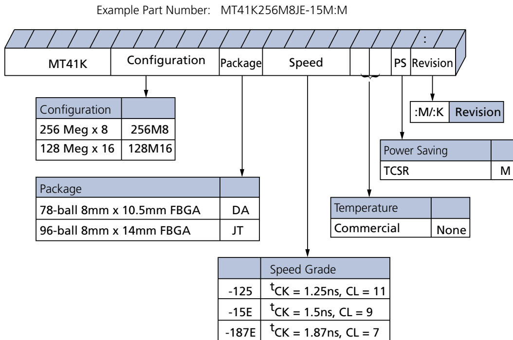
Figure 1: DDR3L-RS Part Numbers
