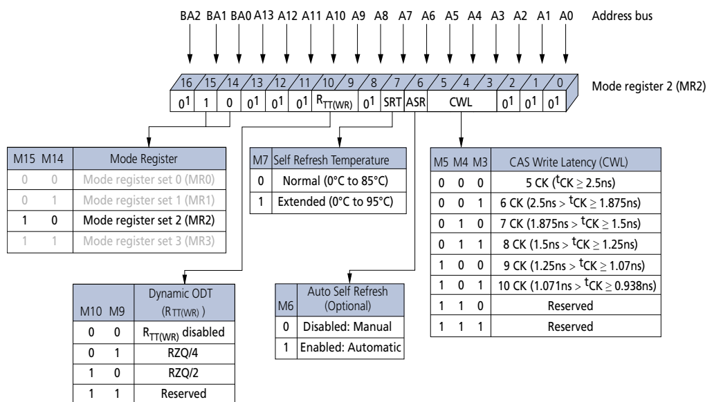
Figure 6: Mode Register 2 (MR2) Definition
