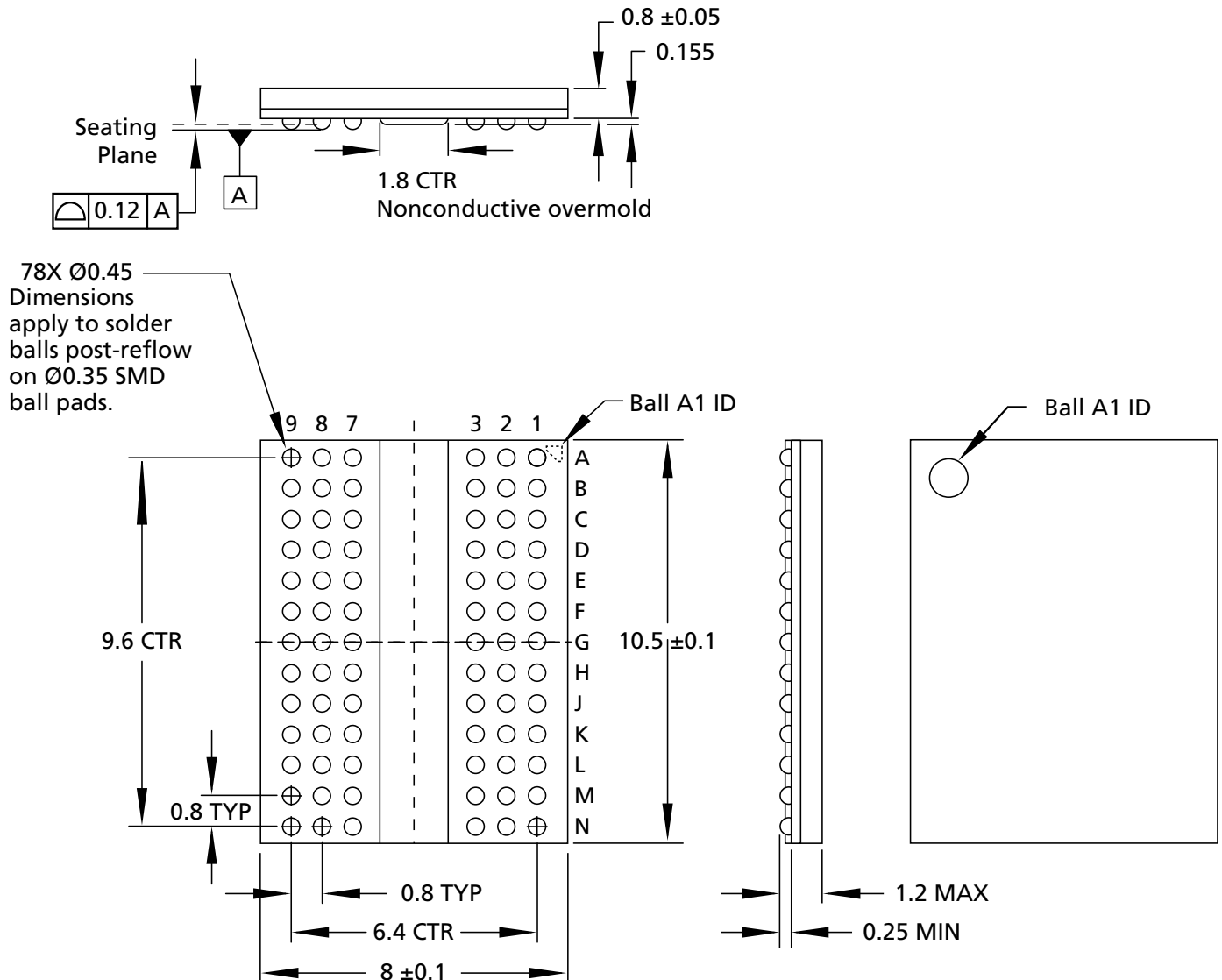
Figure 4: 78-Ball FBGA – x4, x8; Die Rev. M, K (DA)
