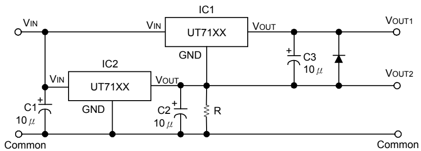
Dual supply
