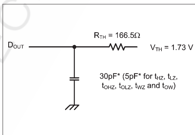
Figure 2. Thevenin Equivalent
