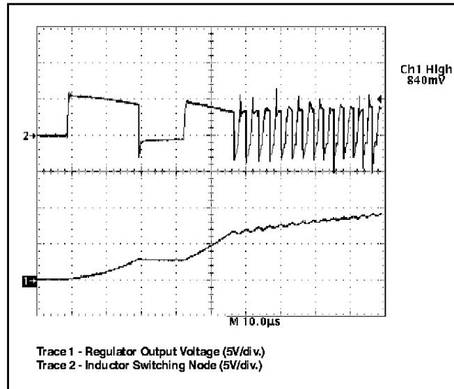
Figure 4: CS-5157 demonstration board enable startup waveforms.
