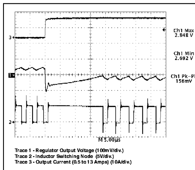
Figure 8: CS-5157 demonstration board response to 13A load turn on (output set for 2.8V). Upon completing a normal off time, the V^{2TM} control loop immediately connects the inductor to the input voltage, providing 100% duty cycle. Regulation is achieved in less than 20μs.
