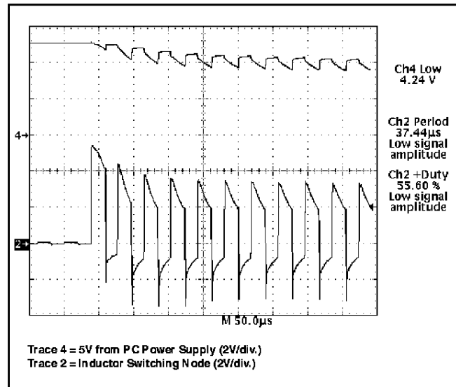
Figure 11: Startup with regulator output shorted.
