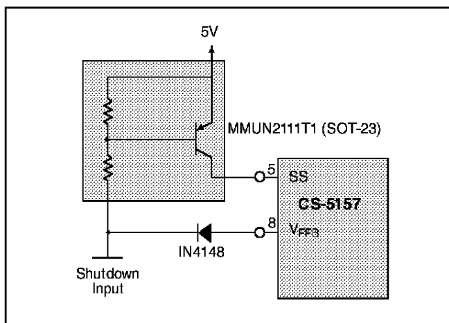
Figure 14: Implementing shutdown with the CS-5157.
