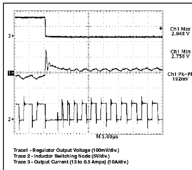
Figure 9: CS-5157 demonstration board response to 13A load turn off (output set for 2.8V). V^{2TM} control topology immediately connects inductor to ground, providing 0% duty cycle. Regulation is achieved in less than 10μs.
