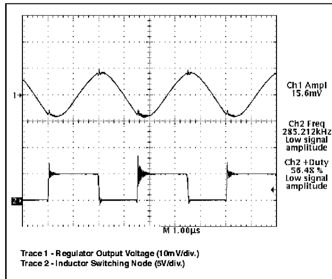
Figure 5: Peak-to-peak ripple on V_{OUT} = 2.8V , I_{OUT} = 0.5A (light load).
