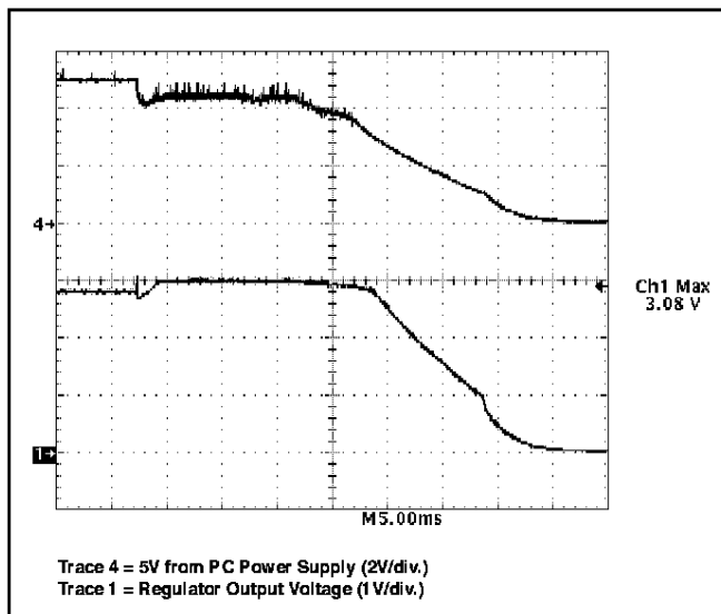
Figure 13: OVP response to an input-to-output short circuit by pulling the input voltage to ground.
