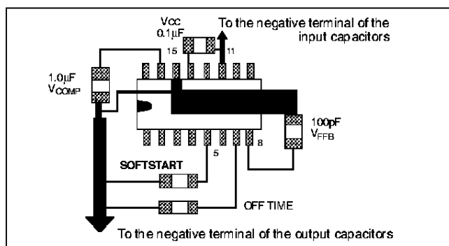
Figure 20: Layout Guidelines
