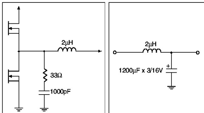
Figure 18: Filter components
