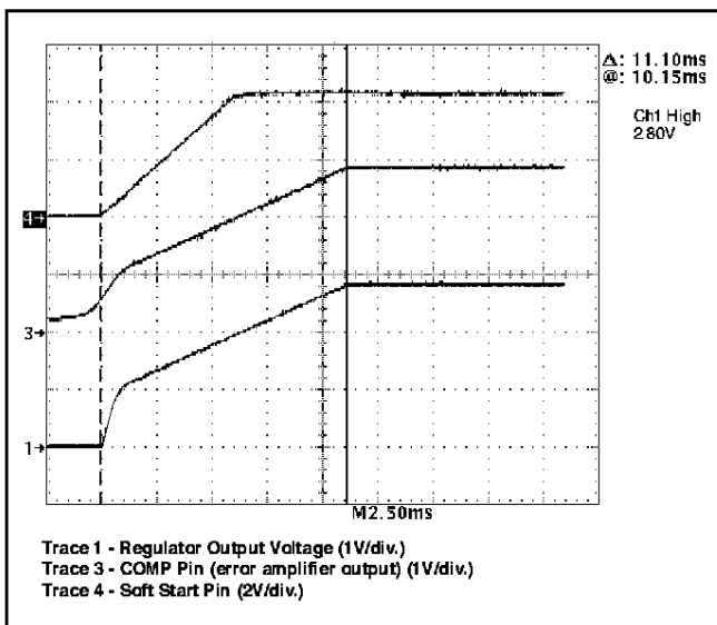
Figure 3 CS-5157 demonstration board startup waveforms.
