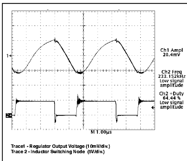
Figure 6: Peak-to-peak ripple on V_{OUT} = 2.8V , I_{OUT} = 13A (heavy load).
