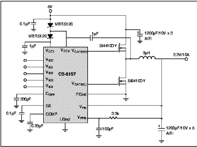
Figure 21: 5V to 3.3V/10A converter.
