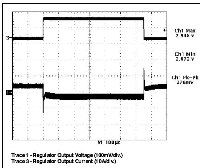
Figure 7: CS-5157 demonstration board response to a 0.5 to 13A load pulse (output set for 2.8V).
