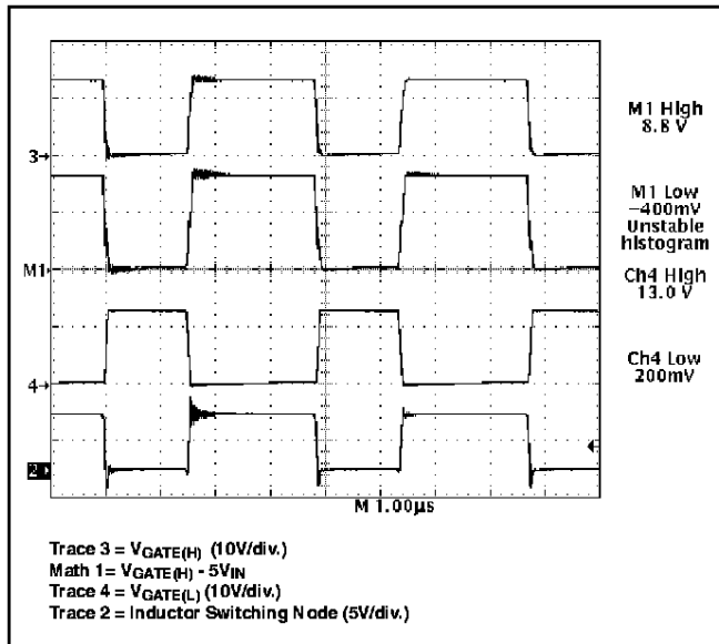
Figure 17: CS-5157 gate drive waveforms depicting rail to rail swing.
