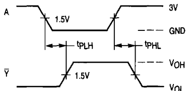
Figure 1. Switching Waveforms
