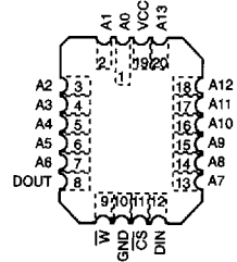
Pinout LCC 20 pins (top view)
