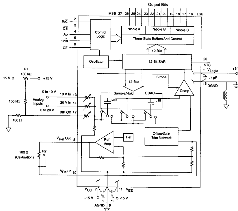
Figure 11 - Unipolar Input Connections
