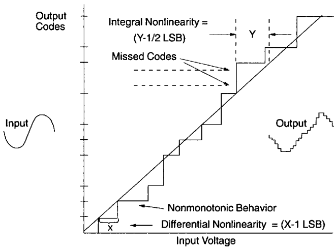
Figure 7 - Quantizing Error
