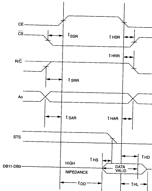
Figure 2 - Read Mode Timing Diagram
