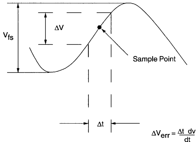
Figure 10 - Aperture Uncertainty
