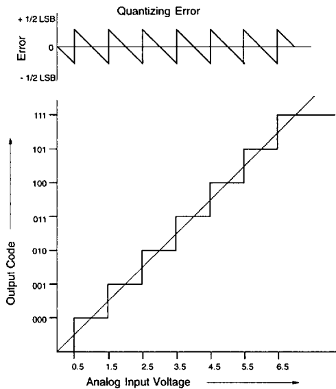
Figure 7 - Quantizing Error
