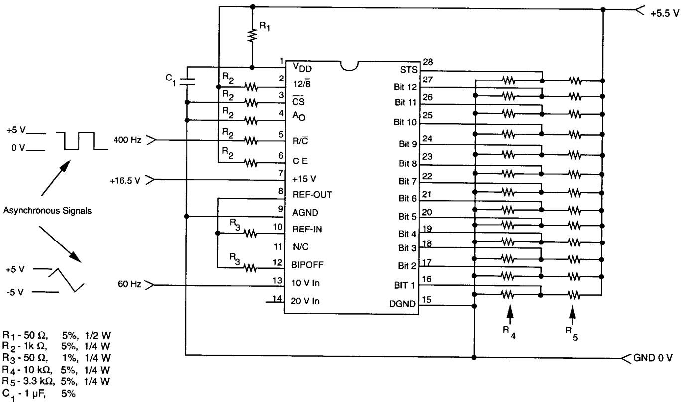
Figure 15 - Burn-In Schematic
