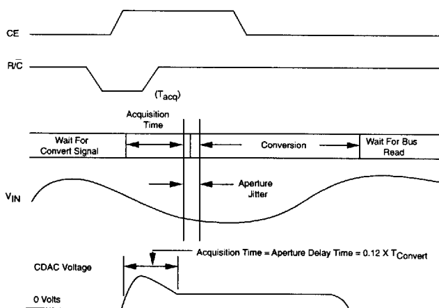
Figure 8 - Sample-and-Hold Function
