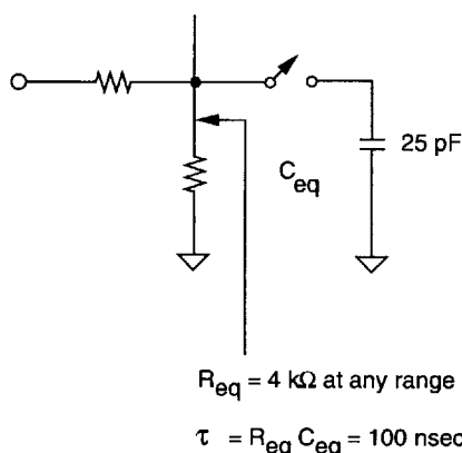
Figure 9 - Equivalent SPT774 Input Circuit
