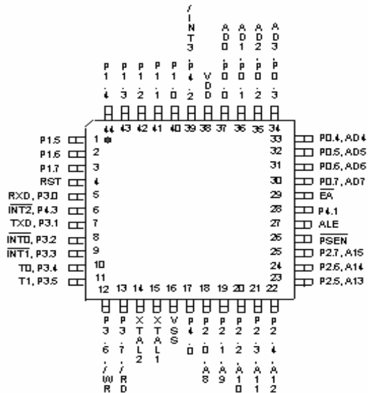
44-Pin QFP
