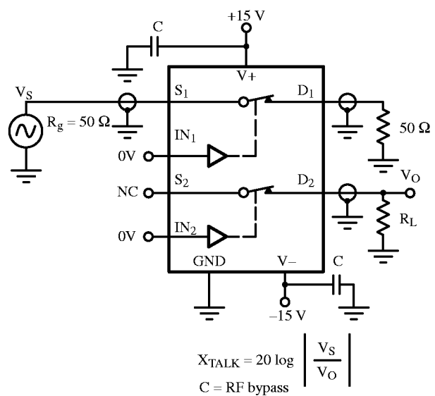
Figure 5. Channel-to-Channel Crosstalk
