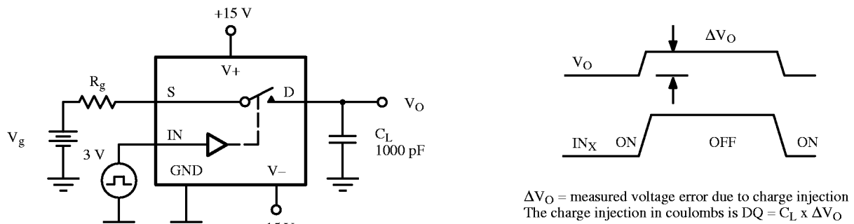
Figure 3. Charge Injection
